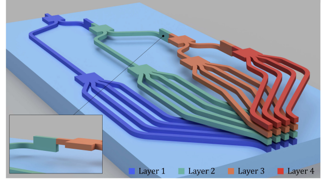
Fig. 3. Concept of 2D OPAs based on PolyBoard PICs with multiple waveguiding layers and vertical MMI couplers for light coupling between adjacent layers. End-fire single-mode waveguides serve as optical AEs at the end-facet of the PolyBoard PIC (cladding material omitted for clarity). A 4 \times 4 OPA is shown as example. Alternatively, an intermediate layer (Layer 2 or 3) can be also used as the seed layer. Vertical couplers that couple directly the seed to the target layer without involving the intermediate ones can be also used. Inset: Close view of a vertical MMI coupler followed by a lateral one.
